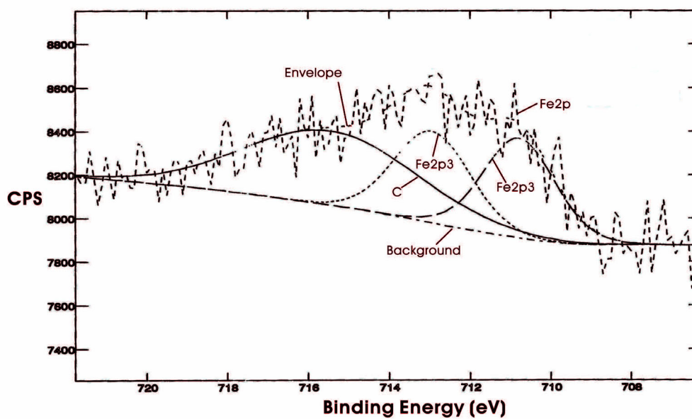
B: XPS spectra of the Fe 2p_{2/3} region for resin/ Fe^{3+} catalyst after use for degradation of 0.2mM MG by 0.5 mM H_2O_2 (total volume 50ml, initial pH 6.0).
