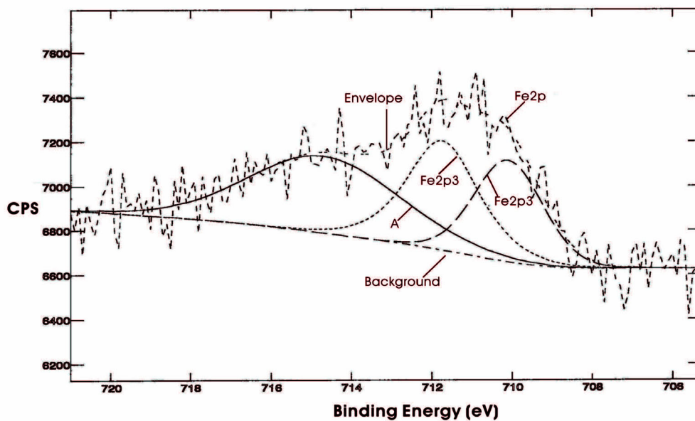
A: XPS spectra of the Fe 2p_{2/3} region for resin/ Fe^{3+} catalyst before use. The Gaussian-Lorentzian fitting of the experimental curves is also shown.
